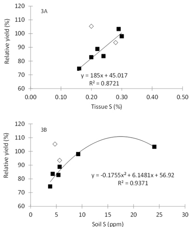
Figure 3: Tissue S content (A) and 0.01 mol L -1 CaCl 2 extractable soil S (B) as predictors for relative yield of alfalfa (the ratio of yield without and yield with the addition of 150 lbs S/acre). The open diamonds indicate two locations with suboptimal pH (6.2 or lower). Adapted from Ketterings et al. (2012).
